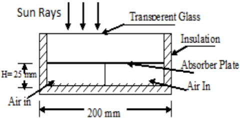
A — Cross Section of wooden duct
