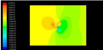
Contours of Static Pressure (pascal) Mar 16, 2019 FLUENT 6.3 (2d, dp, p6mm, s1e1)
