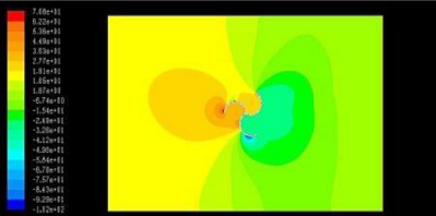
Contours of Static Pressure (pascal) Mar 16, 2019 FLUENT 6.3 (2d, dp, p6mm, s1e1)
