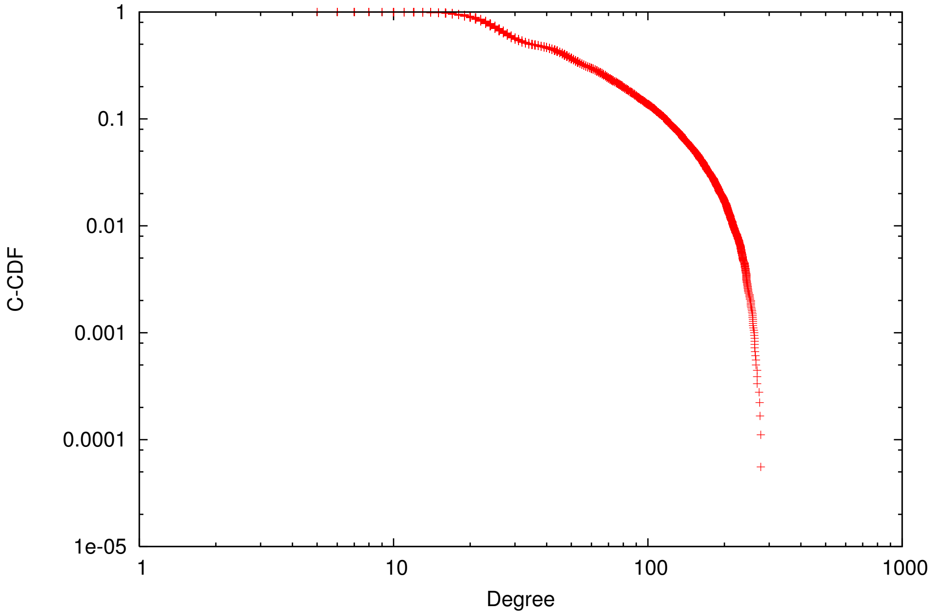
C-CDF of Degree Distribution
